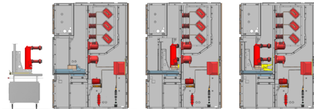
External Transfer of Switching Device (Example)
