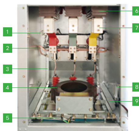
1250A Cable Connection Compartment (Example)
