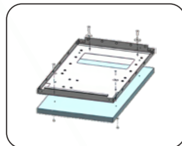
Installation Method C – installation on bracket lifted plate
