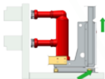
Disconnected position
